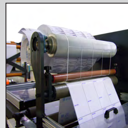
Snowball waste rewind
